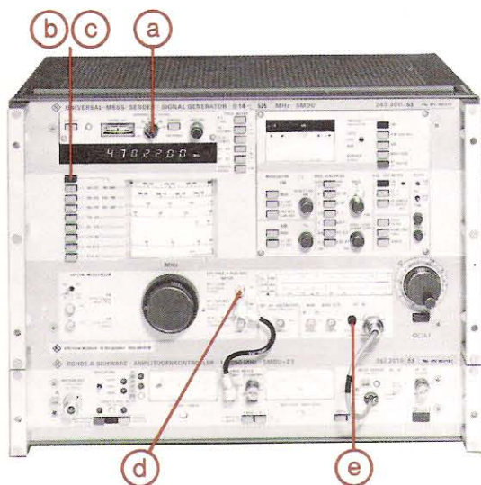
Figure 2 SMDU model 52 or 53, a single-cabinet test assembly for AM and FM radiotelephones
