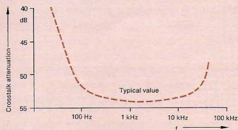
Channel crosstalk in stereo modulation as a function of modulation frequency
