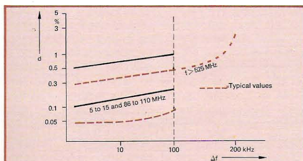
FM modulation distortion measured with a distortion-free modulating signal of 15 Hz to 53 kHz as a function of frequency deviation
