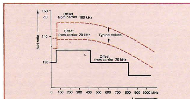
Figure 9 Signal-to-noise ratio with 1-Hz measuring bandwidth for various carrier offsets as a function of carrier frequency
