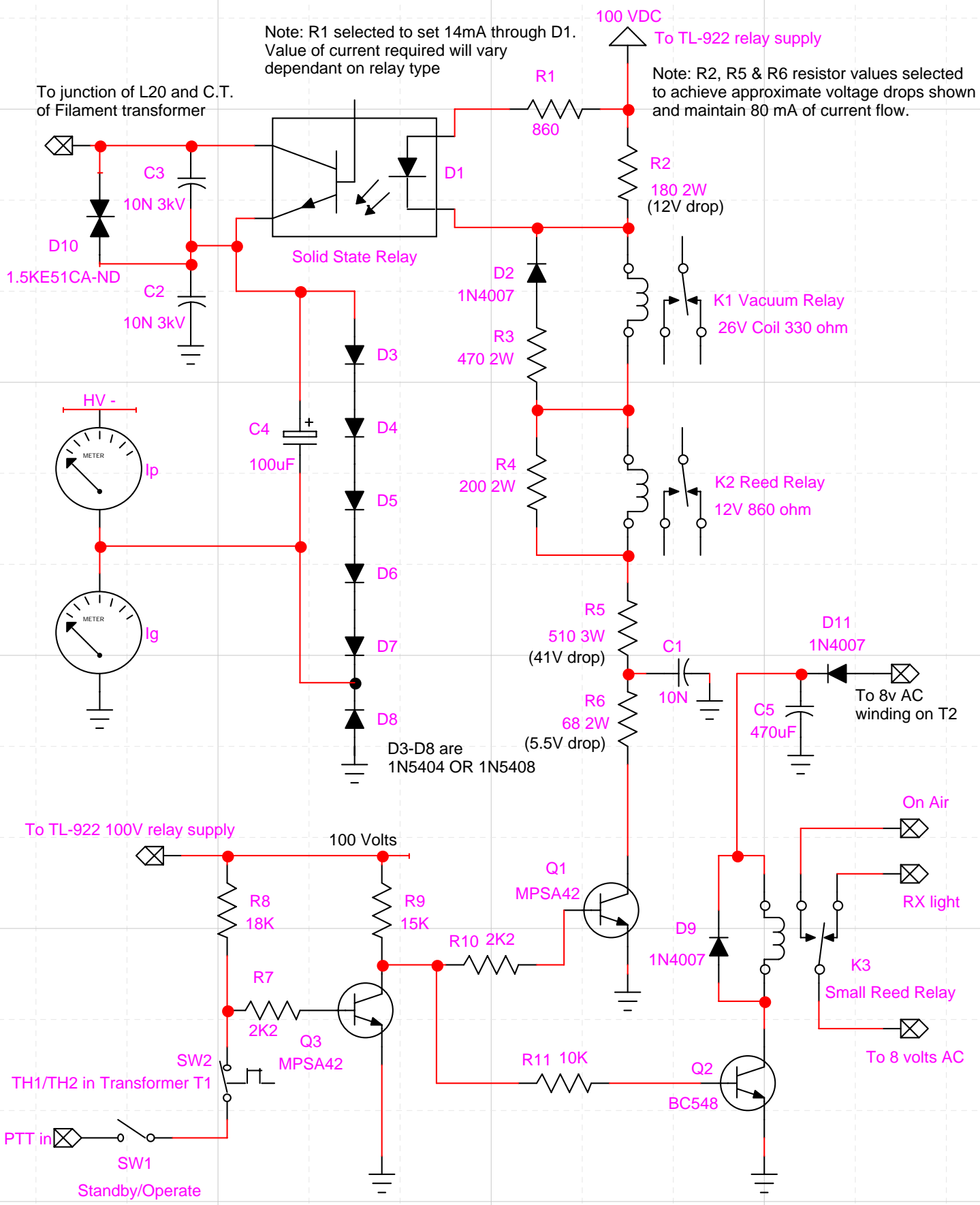
VK2FC' version of QSK for the TL-922 Linear Amplifier Last updated in April 2008
